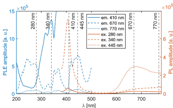
Fig. 7 PLE and PL spectra of the Li 2 MnCl 4 :Eu 2+ (1%) sample. The excitation and emission wavelengths are indicated by dashed lines. The high intensity at around 200 nm is due to overcorrection.
