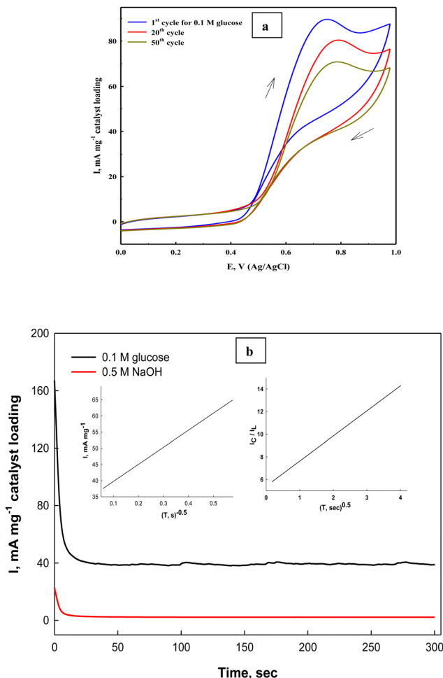
Fig. 12 (a) Repeated cyclization of the Ni(II)-SB/C electrode in 0.5 M NaOH + 0.1 M glucose, and (b) chronoamperometry of the same electrode at 0.72 V and the inset plots represent I and I_C/I_L and square root of time (left) and the relationship of I_C/I_L and square root of time (right).
