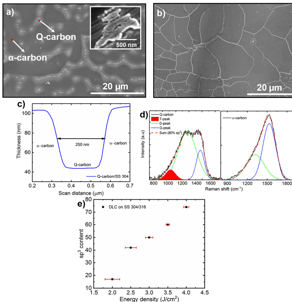
Fig. 9 (a) SEM image demonstrating the formation of Q-carbon on 304 SS, inset shows high-resolution image of Q-carbon in \alpha -matrix, (b) SEM image of Q-carbon, (c) surface roughness measurement of Q-carbon, (d) Raman spectra of Q- and \alpha -carbon, and (e) correlation between sp^3 content of the DLC as a function of laser energy density used during deposition. 159 Reproduced from ref. 154 with permission from Elsevier, copyright 2020.
