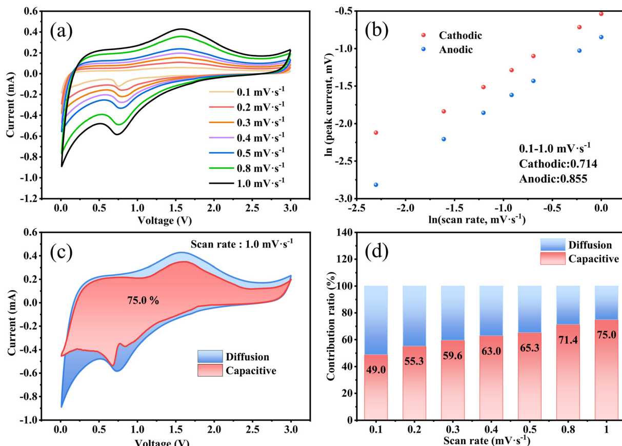
Fig. 5 CV curves of the Fe 3 O 4 QDs@C/RGO composite electrode from 0.1 to 1.0 mV s -1 (a), the ln( i )-ln( v ) plot (b), the capacitive contribution of the Fe 3 O 4 QDs@C/RGO composite electrode at 1 mV s -1 (c) and the pseudocapacitive contribution ratios at different scanning rates (d).
