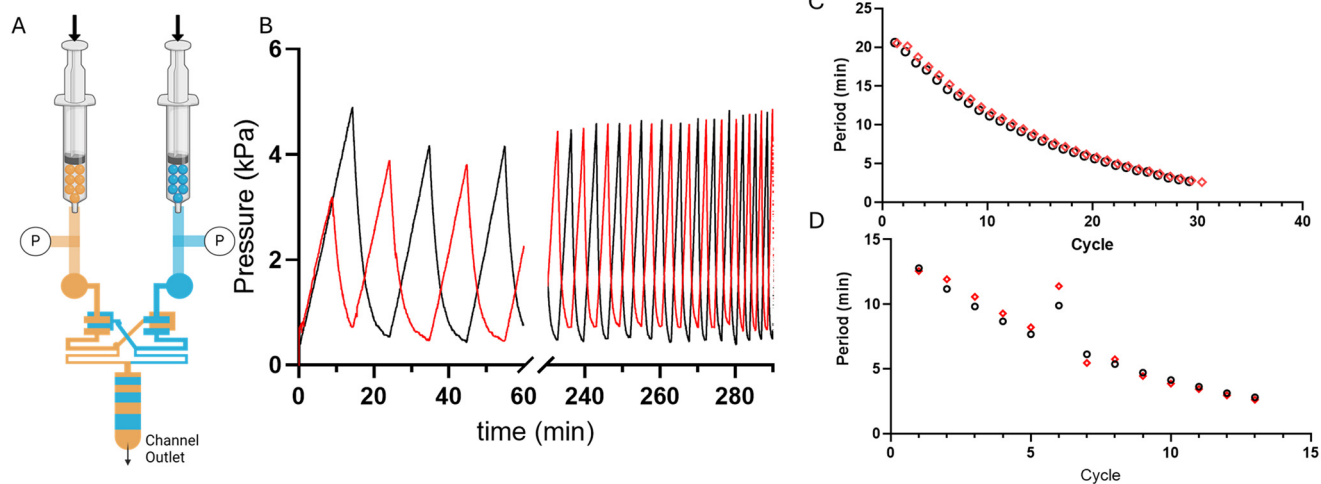
Fig. 4 Forced-air oscillators have decreasing periods over time as the syringes' fluid volumes reduce and the syringe pump continues to run. Even though the oscillation period decreases, the oscillatory behavior is persistent. A) A representative schematic of a microfluidic oscillator being driven by gas packets. Two pressure sensors, the circles with (P), upstream of the microfluidic oscillator record the pressure profiles of each fluid line. B) A 20 \mu\text{m} membrane oscillator system being driven by two 60 mL syringes at a 200 \mu\text{L min}^{-1} flow rate. Graphed pressure data is split to demonstrate the stark difference in period over the first 60 minutes compared to the (approximately) final 60 minute at the end of the run. C) Period decreases with each oscillation cycle for the 20 \mu\text{m} membrane oscillator and D) a 100 \mu\text{m} membrane oscillator, which was run at 500 \mu\text{L min}^{-1} .
