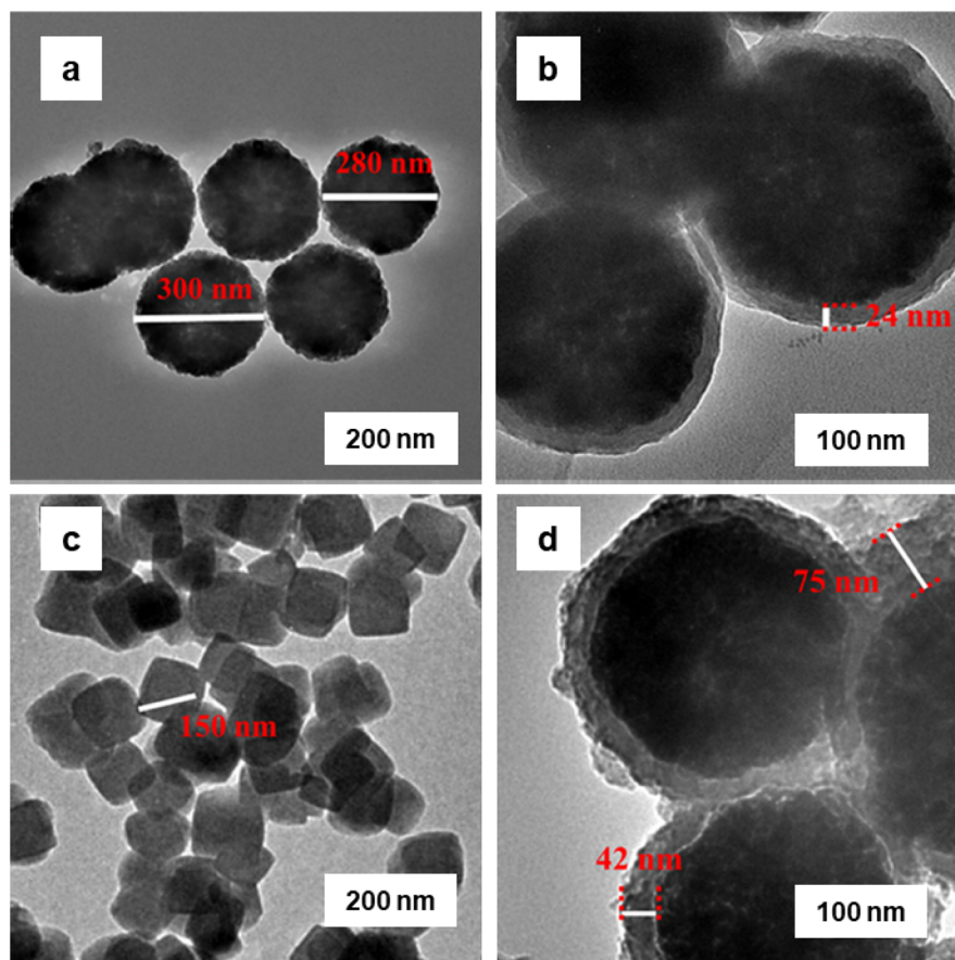
Fig. 65 TEM images of (a) \text{Fe}_3\text{O}_4 ; (b) \text{Fe}_3\text{O}_4@\text{PDA} ; (c) \text{UiO-67-bpydc} ; and (d) \text{Fe}_3\text{O}_4@\text{UiO-67-bpydc} . Reproduced with permission from ref. 418 Copyright 2021, American Chemical Society.
