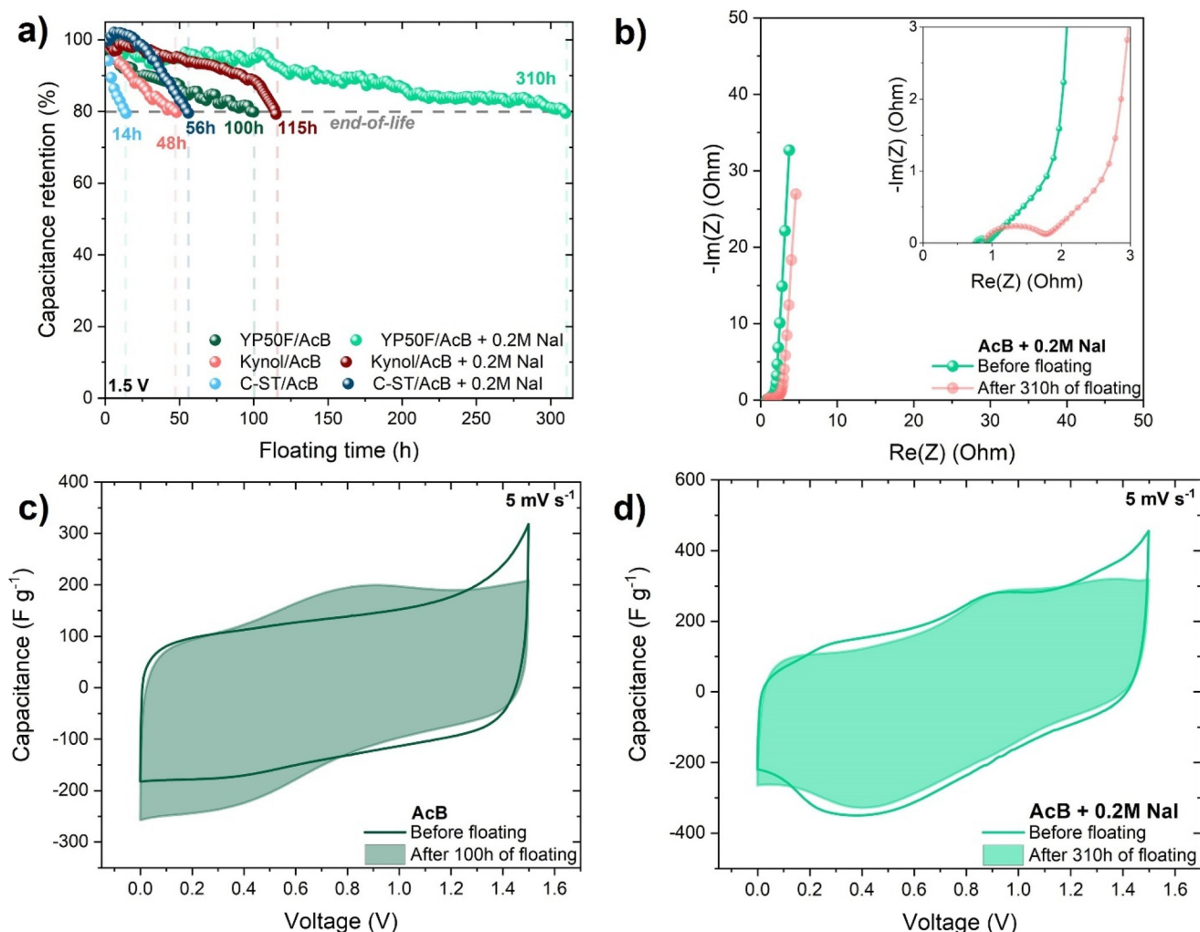
Fig. 4 (a) Capacitance retention of different microporous carbons (YP50F, Kynol, and C-ST) based ECs operating in acetate buffer with and without 0.2 mol L^{-1} NaI additive during the floating test (at 1.5 V). (b) Nyquist plots obtained from YP50F-based ECs operating in acetate buffer + 0.2 mol L^{-1} NaI before and after 310 h floating test. Cyclic voltammogram at 5 mV s^{-1} recorded for (c) acetate buffer before and after 100 h floating test; (d) acetate buffer + 0.2 mol L^{-1} NaI before and after 310 h floating test.
