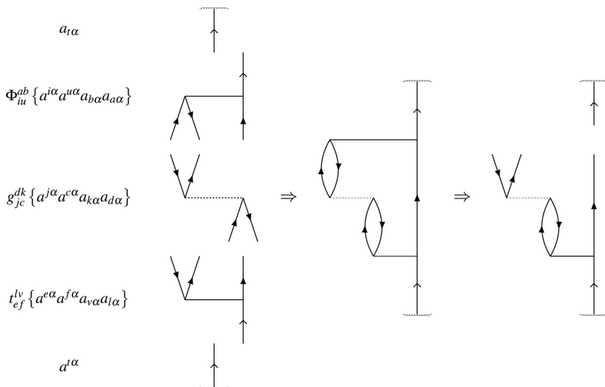
Fig. 2 Goldstone diagram construction representing the automated generation of the residual term r_{ab}^{iu} = g_{jc}^{dk} t_{ef}^{lv} \delta_t^i \delta_k^f \delta_b^c \delta_a^j \delta_d^e \delta_v^t .
