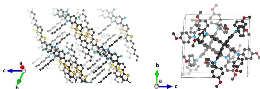
Fig. 2 Minimum-energy crystal structure calculated at the PBEsol level of theory for IDIDF (left) and spiro-OMeTAD (right). Color coding: C in black, S in yellow, N in blue, O in red and F in cyan. H atoms are omitted for clarity.
