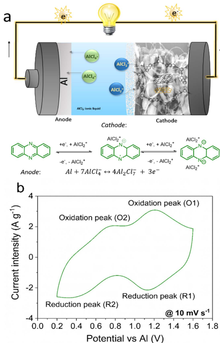
Fig. 2 (a) Scheme of the aluminium-phenazine battery during discharge and general redox working mechanism of the phenazine unit and Al reactions. (b) CV recorded at 10\ mV\ s^{-1} illustrating the two sequential one-electron and one- AlCl_2^+ redox reaction steps.
