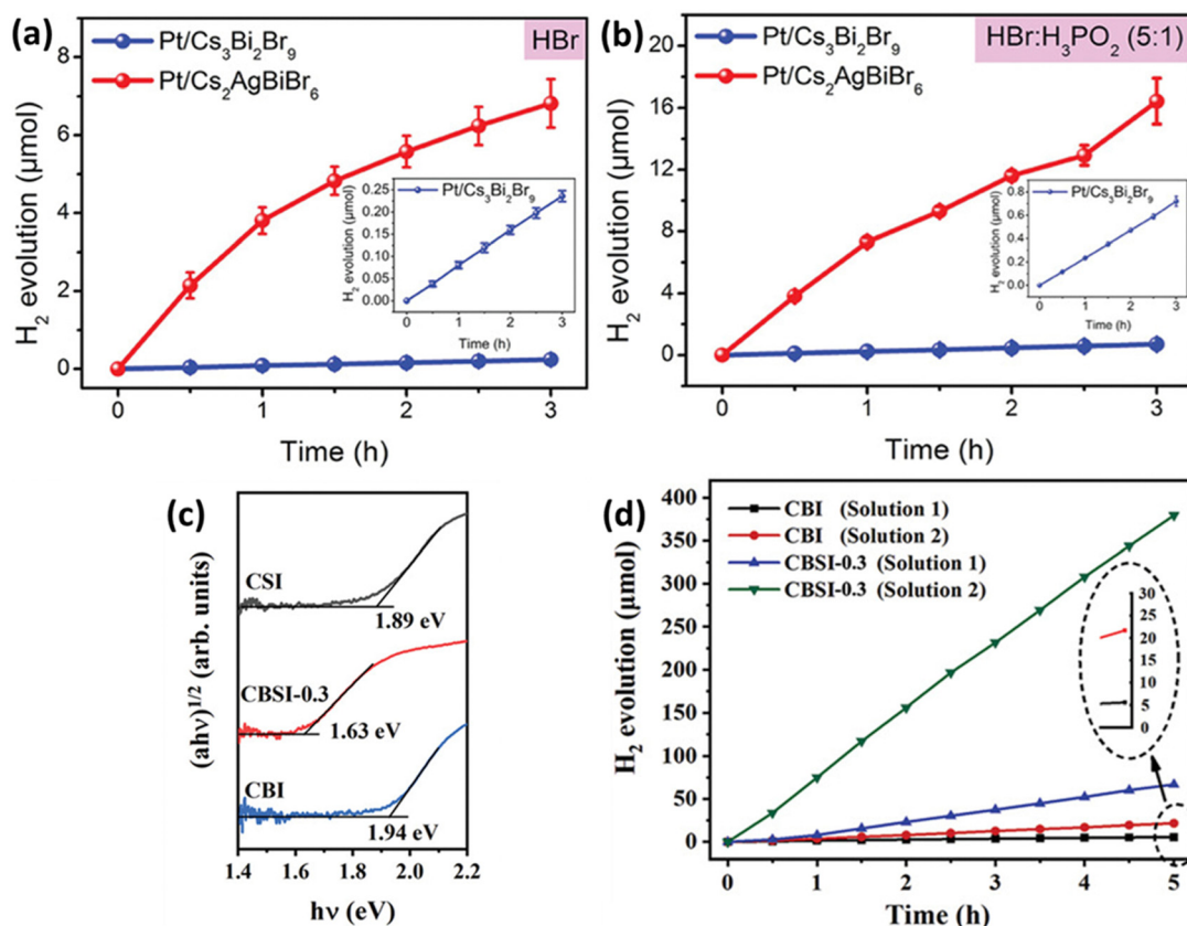
Fig. 5 Hydrogen evolution performance of Pt/ \text{Cs}_3\text{Bi}_2\text{Br}_9 and Pt/ \text{Cs}_2\text{AgBiBr}_6 in aqueous solutions of (a) HBr and (b) HBr/ \text{H}_3\text{PO}_2 . 85 Reproduced with permission from ref. 85 Copyright © 2020 Wiley-VCH Verlag GmbH & Co. KGaA, Weinheim. (c) Optical absorption spectra of \text{Cs}_3\text{Bi}_2\text{I}_9 (CBI), \text{Cs}_3\text{Sb}_2\text{I}_9 (CSI), and \text{Cs}_3\text{Bi}_{2x}\text{Sb}_{2-2x}\text{I}_9 (CBSI-0.3). (d) Comparative analysis of the hydrogen evolution activity between CBI and CBSI-0.3 in Solution 1 and 2. 86 Reproduced with permission from ref. 86 Copyright © 2020 Wiley-VCH GmbH.
