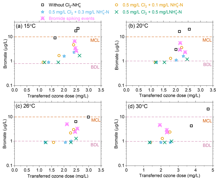
Fig. 5 Effect of transferred ozone dose on effluent bromate concentrations under different \text{Cl}_2\text{-NH}_4^+\text{-N} dosing scenarios at (a) 15 °C, (b) 20 °C, (c) 26 °C, and (d) 30 °C. The symbols in magenta represent results from challenge tests conducted with additional 40 \mu\text{g L}^{-1} bromide spiked into raw water, to increase the influent bromide from 80 \mu\text{g L}^{-1} to 120 \mu\text{g L}^{-1} (confirmed with laboratory analysis). MCL = maximum contaminant limit = 10 \mu\text{g L}^{-1} . BDL = below detection limit = of 1 \mu\text{g L}^{-1} .
