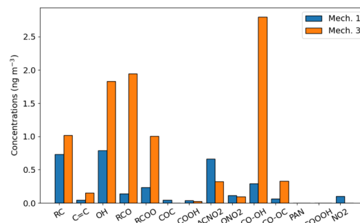
Fig. 6 Functional groups simulated in the average toluene SOA concentrations over Greater Paris in May–June 2014, using rdc. Mech. 1 and rdc. Mech. 3: alkyl (RC), double C bound ( \text{C}=\text{C} ), alcohol (OH), carbonyl (RCO), ester (RCOO), ether (COC), acid (COOH), nitroaromatic (ACNO2), nitrate (ONO2), hydroperoxide ( \text{CO}-\text{OH} ), peroxide ( \text{CO}-\text{OC} ), peroxyacetyl nitrates (PAN), peroxyacetyl acid (COOOH), nitroalkyl (NO2).
