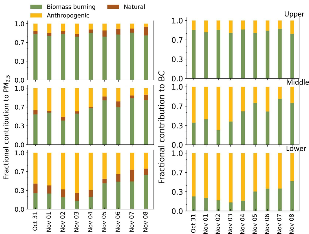
Fig. 4 Fractional contributions of biomass burning, natural and anthropogenic emissions to daily mean modelled surface PM 2.5 (left panels) and BC (right panels) averaged over the upper, middle and lower IGP regions shown in Fig. 1 for each day of the extreme pollution event (31 Oct–8 Nov 2016).
