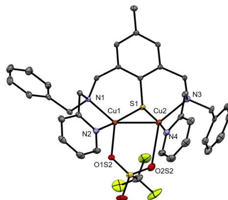
Fig. 3 ORTEP diagram (30% probability) for the dicationic unit of 6 . H-atoms are omitted for clarity. Selected bond distances ( \text{\AA} ): \text{Cu1-Cu2} 2.5475(5) , \text{Cu1-S1} 2.1798(8) , \text{Cu2-S1} 2.1661(8) , \text{Cu1-N1} 2.043(2) , \text{Cu1-N2} 1.959(3) , \text{Cu1-O1S2} 2.176(2) , \text{Cu2-N3} 2.114(3) , \text{Cu2-N4} 1.945(3) , \text{Cu2-O2S2} 2.674(9) ; see Tables S1–S3, ESI†.
