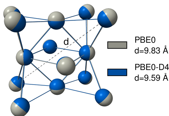
Fig. 8 PBE0/def2-SVP (grey) and PBE0-D4/def2-SVP (blue) optimized \text{No}_{14} -cluster. PBE0-NL/def2-SVP is hidden for better visibility, however, the result is very similar to the D4 result with d=9.55 Å. The calculated diagonal distance is shown as the dashed black line.
