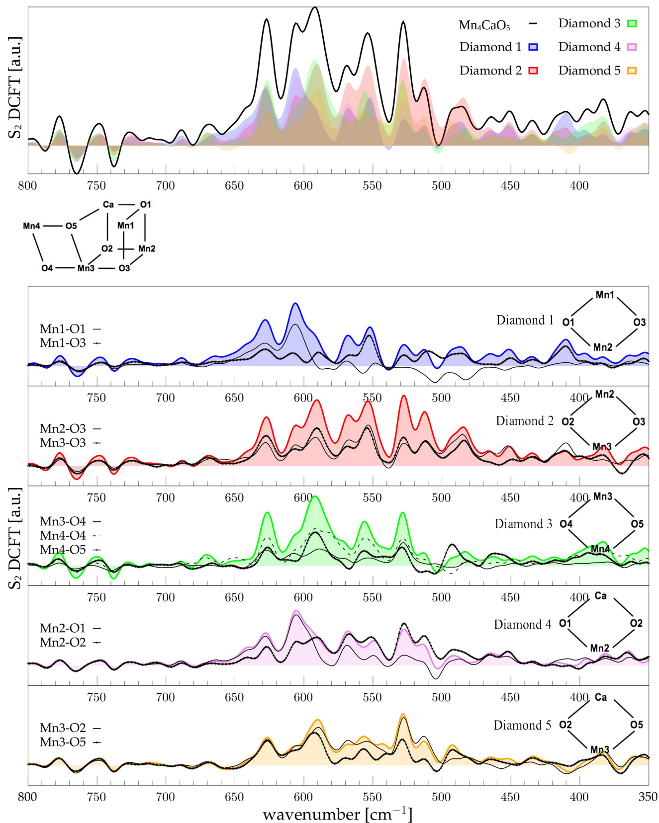
Fig. 5 The top panel displays the FT of the dipole correlation for the \text{Mn}_4\text{CaO}_5 cluster (black line) and the diamond subunits (colored areas) in the S_2 state. In the lower panels, the FT of the dipole correlation for each Mn-O moiety is compared with the same analysis for the diamond in which it is contained.
