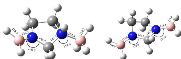
Fig. 3 Optimized structures of the two dehydrogenated counterparts of IMBB ( MDIMBB and DDIMBB ) with geometrical parameters at M06-2X/cc-pVQZ by the removal of H 2 above then below the ring.
