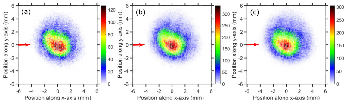
Fig. 3 Velocity map images of Cl − ions (central time slice) taken for (a) 0.1 eV, (b) 0.2 eV and (c) 0.5 eV incident electron energies around the A 1 resonance. The red arrows indicate the incident electron beam direction.
