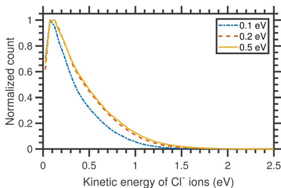
Fig. 4 Kinetic energy distributions of Cl − ions arising from the DEA to CCl 4 for three different incident electron energies, as shown in the figure, around the A 1 resonance.
