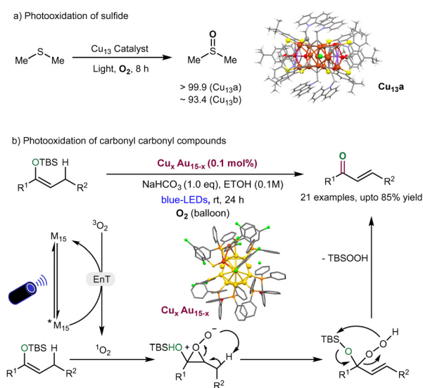
Fig. 7 (a) Quasi-structurally isomeric \text{Cu}_{13} NCs catalyzed photocatalytic sulfide oxidation. (b) Photo-oxidation of carbonyl compounds by \text{Cu}_x\text{Au}_{15-x} NCs.
