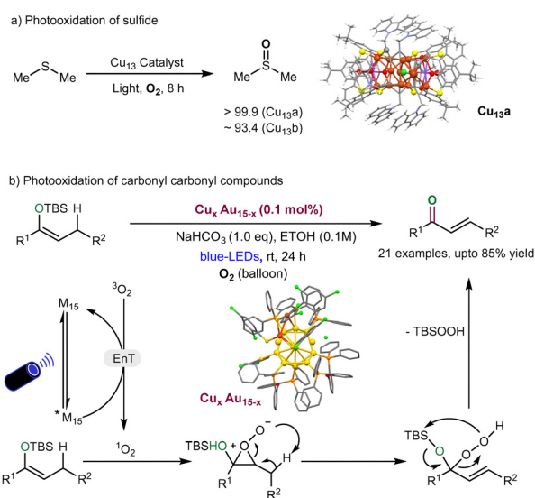
Fig. 7 (a) Quasi-structurally isomeric \text{Cu}_{13} NCs catalysed photocatalytic sulfoxidation of sulfides. (b) Photo-oxidation of carbonyl compound derivatives by \text{Cu}_x\text{Au}_{15-x} NCs.
