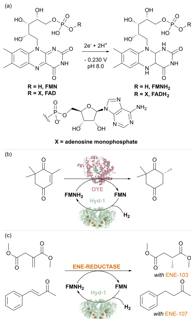
pharmaceutical synthesis, particularly where there are already biocatalytic steps in the synthesis. We have also made use of the intact soluble hydrogenase from C. necator , in vitro , for recycling the deuterated cofactor NAD 2 H during the synthesis of isotopically-labelled amino acids to use in the expression of labelled proteins for NMR structural study. 41
