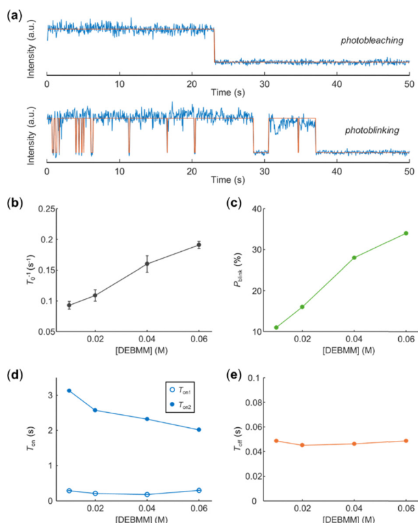
Fig. 2 (a) Photobleaching and photoblinking trajectories of single EYs in DEBMM. (b)–(e) The effect of DEBMM concentration on (b) photobleaching rate of EY\ T_0^{-1} , (c) percentage of photoblinking EY\ P_{\text{blink}} , (d) T_{\text{on1}} and T_{\text{on2}} of photoblinking EYs, and (e) T_{\text{off}} of photoblinking EYs.
