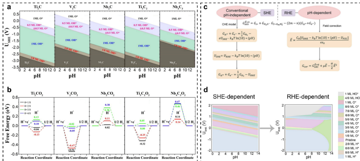
Fig. 8 (a) Calculated surface Pourbaix diagrams of Ti 2 C, V 2 C, Nb 2 C, Ti 3 C 2 , and Nb 4 C 3 ; (b) free-energy evolutions of the HER at different H* coverages ( \theta = 1/8, 2/8, 3/8, \text{ and } 4/8 ) occurring on Ti 2 CO 2 , V 2 CO 2 , Nb 2 CO 2 , Ti 3 C 2 O 2 , and Nb 4 C 3 O 2 under standard conditions. 151 (c) Schematic illustration of the RHE scale-dependent method; (d) calculated classic SHE-dependent and RHE-dependent surface Pourbaix diagrams for Pt(111). 50
