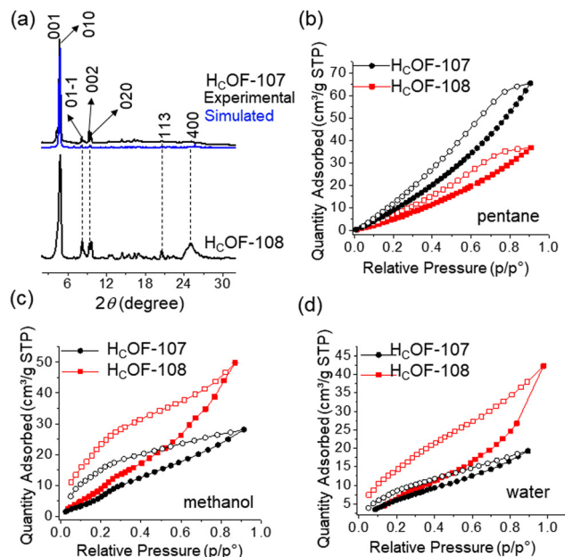
Fig. 4 (a) Simulated ( \text{HcOF-107} ) and experimental PXRD patterns of \text{HcOF-107} and \text{HcOF-108} . (b) Pentane, (c) methanol, and (d) water vapor sorption isotherms (295 K) for \text{HcOF-107} (black) and \text{HcOF-108} (red).
