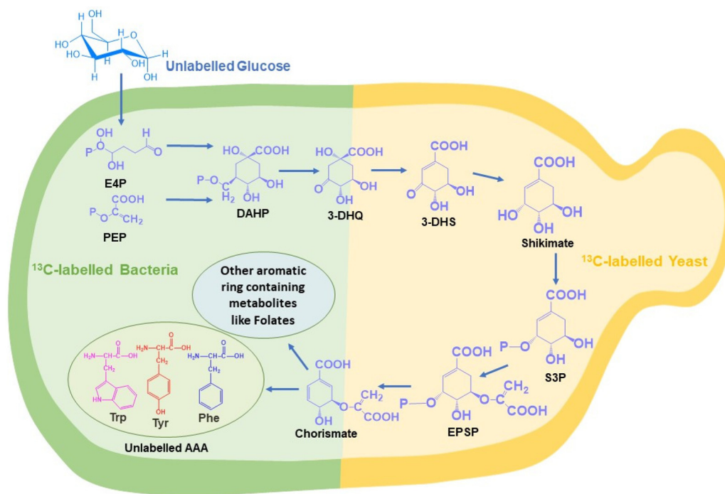
Fig. 1 Reverse labelling of the shikimate pathway occurring in both 13 C-labelled bacteria (green) and 13 C-labelled yeast (yellow) showing the carbon flow from unlabelled glucose to the synthesis of aromatic amino acid and aromatic ring-containing metabolites. (Abbreviation: E4P – erythrose-4-phosphate; PEP – phosphoenol pyruvate; DAHP – 3-deoxy- o -arabino-heprulosonate 7-phosphate; 3-DHQ – 3-dehydroxyquininate; 3-DHS – 3-dehydroshikimate; S3P – shikimate-3-phosphate; EPSP – 5-enolpyruvylshikimate 3-phosphate; Phe – phenylalanine; Tyr – tyrosine; Trp – tryptophan; AAA – aromatic amino acid.)
