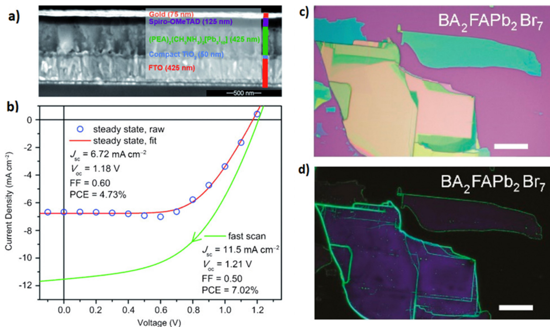
Fig. 21 (a) SEM cross-sectional image and device configuration of planar devices utilizing (PEA) 2 (MA) 2 [Pb 3 I 10 ] as the absorber layer. Scale bar = 500 nm. (b) Current–voltage ( J – V ) curves for the devices fabricated as given in (a). Adapted with permission from ref. 337. (c and d) Optical and PL images of a series of 2D BA 2 FAPb 2 Br 7 lead halide perovskites mechanically exfoliated on SiO 2 /Si substrates. Adapted with permission from ref. 342.
