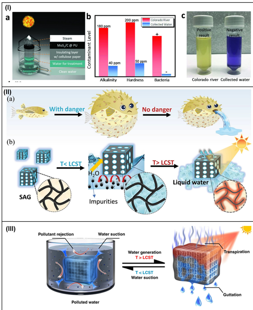
Fig. 13 Wastewater purification via SIWE devices. (I) (a–c) \text{MoS}_2/\text{C} @PU solar steamer – design and performance. Reproduced with permission. 184 Copyright 2018, Wiley-VCH. (II) Design illustration of a solar absorber gel for clean water production. Reproduced with permission. 185 Copyright 2021, Wiley-VCH. (III) Schematic of water treatment of the sunlight-powered purifier (PNPG-F) – the coated PG demonstrates solar–thermal conversion and pollutant rejection. Reproduced with permission. 65 Copyright 2019, Nature.
