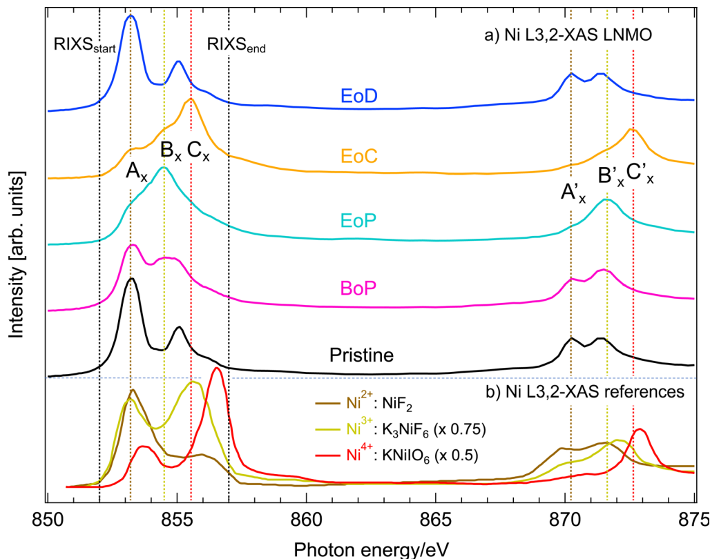
Fig. 4 (a) Ni L 3,2 -edge XAS in PFY mode of Li 1-x Ni 0.44 Mn 1.56 O 4 at different SoC (see Fig. 1). The black dashed, vertical lines mark the incident energy region straddling the L 3 -resonances covered by RIXS. (b) Ni L 3,2 -edge XAS reference spectra for Ni 2+ (NiF 2 ), Ni 3+ (K 3 NiF 6 ), and Ni 4+ (KNiO 6 ), respectively, as reported by Wang et al. 25 with a respective intensity scaling factor of 0.75 and 0.5 for Ni 3+ and Ni 4+ . The colored dashed, vertical lines are labelled to identify salient spectral features at the Ni L 3,2 -resonances.
