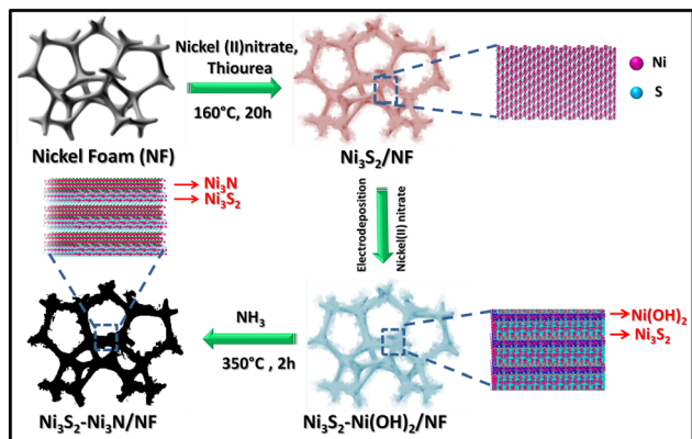
Scheme 1 The synthesis strategy of the \text{Ni}_3\text{S}_2\text{-Ni}_7\text{N/NF} catalyst.
