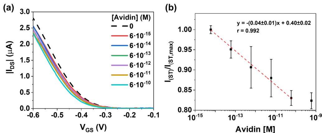
Fig. 4 (a) Transfer characteristics ( V_{DS} = -0.1 V) of an EGOFET employing as gate electrode a CGE with collected biotin-AuMNP previously incubated in a PBS solution of different AV concentrations. The dashed curve represents the transfer after the exposition of the CGE with collected biotin-AuMNP to a reference PBS solution. (b) Relative I_{DS} (at V_{GS} = -0.6 V) vs. AV concentration plot and the calibration.
