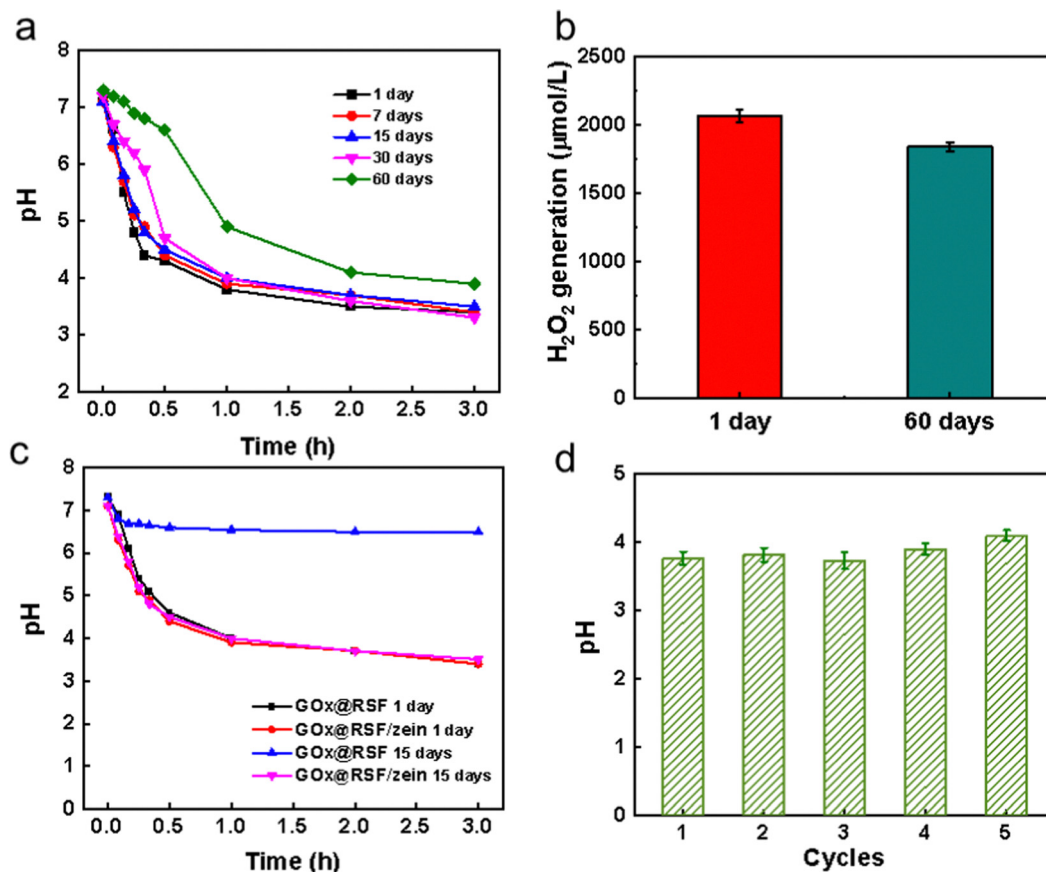
Fig. 3 The stability of GOx@RSF/zein nanospheres. (a) pH change with the reaction time after a different storage period (glucose solution: 1 \text{ mg mL}^{-1} ), (b) \text{H}_2\text{O}_2 generation after 1 day and 60 days of storage, (c) pH change compared with GOx@RSF nanospheres, and (d) pH value during different cycles.
