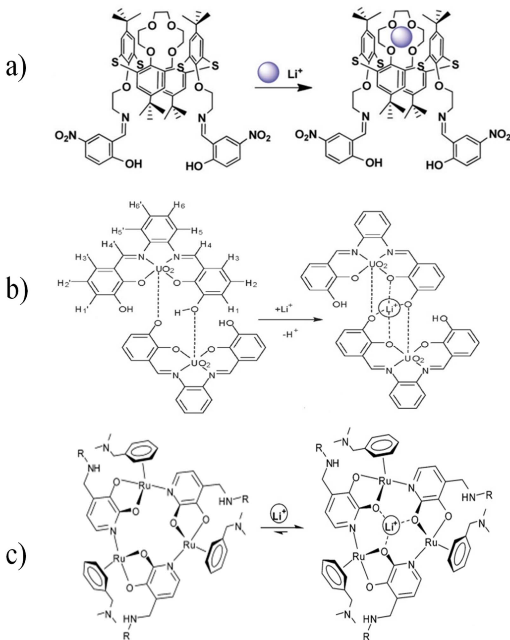
Fig. 18 Mechanism of \text{Li}^+ ion adsorption by (a) thiacalix[4]crown (Reproduced with permission from ref. 129. Copyright 2023, Royal Society of Chemistry), (b) salophen- \text{UO}_2 homodimeric complex (Reproduced with permission from ref. 130. Copyright 2023, American Chemical Society), and (c) ruthenium-based metallacrown complex (Reproduced with permission from ref. 131. Copyright 2023, Royal Society of Chemistry).
