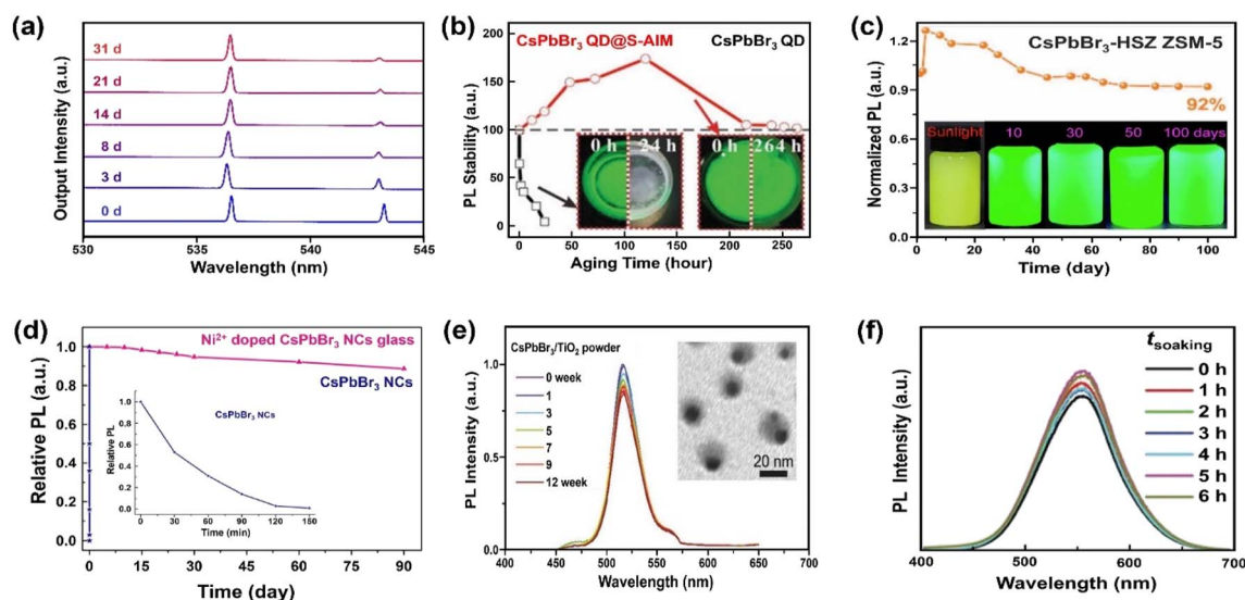
Fig. 6 Stabilizing MHPs by using inorganic materials. (a) Time-dependent normalized lasing spectra of the ALD Al 2 O 3 coated CsPbBr 3 nanoplate after being immersed in water for 1 month. Adapted from ref. 158. Copyright 2020 American Chemical Society. (b) PL intensity evolution over CsPbBr 3 QDs and CsPbBr 3 QDs@superhydrophobic aerogel inorganic matrix (S-AIM) completely immersed in water with time. Adapted from ref. 163. Copyright 2020 John Wiley and Sons. (c) PL stability of CsPbBr 3 -HSZ ZSM-5-700 composites when exposed in water and luminescent photographs of CsPbBr 3 -HSZ ZSM-5-700 composite immersed in water for various time (5 mg mL -1 ). Adapted from ref. 175. Copyright 2022 Elsevier. (d) The change in relative PL of Ni 2+ doped CsPbBr 3 NCs glass and CsPbBr 3 NCs in water (inset: enlarged the change of PL with CsPbBr 3 NCs in water). Adapted from ref. 177. Copyright 2019 Elsevier. (e) The relative PL intensity of CsPbBr 3 /TiO 2 NCs after immersing in Milli-Q water (0–12 weeks), inset shows a TEM image of CsPbBr 3 /TiO 2 NCs after immersing in Milli-Q water for 12 weeks. Adapted from ref. 181. Copyright 2017 John Wiley and Sons. (f) Normalized PL spectra of Cs 2 Sn 0.89 Te 0.11 Cl 6 versus different soaking time. Adapted from ref. 180. Copyright 2020 John Wiley and Sons.
