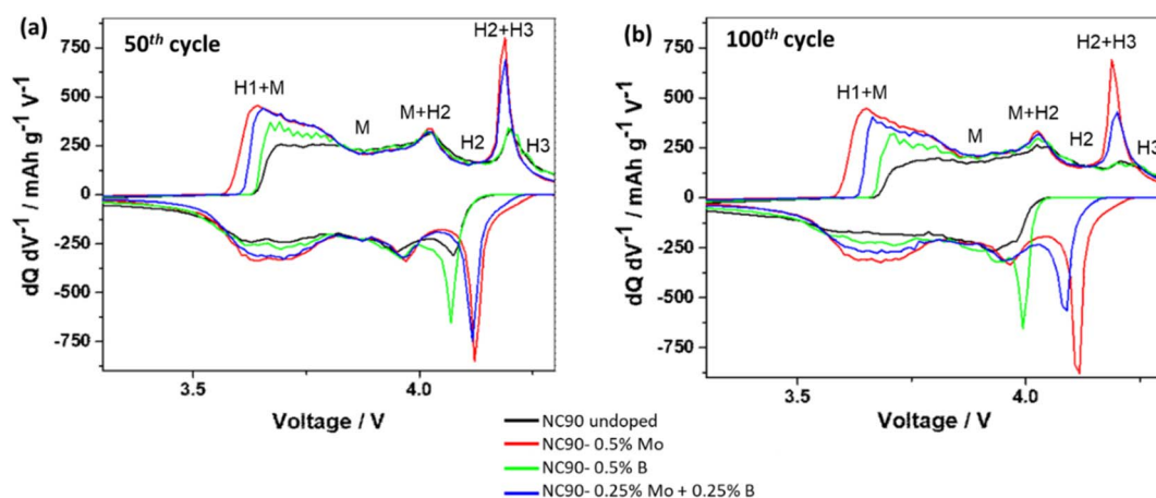
Fig. 7 Differential capacity ( dQ/dV ) vs. potential ( V ) plots of electrodes comprising NC90 undoped and doped materials, as indicated, measured at cycle 50 th (a) and 100 th (b) in half-cells vs. lithium anodes (LP57 solutions, 1C rate, 25 °C). Indicated are hexagonal H and monoclinic M phases and their possible multistep structural transitions in NC90 electrodes upon charge/discharge, as it is well established in the literature (see, for instance: refs. 18, 68, 39 and 44).
