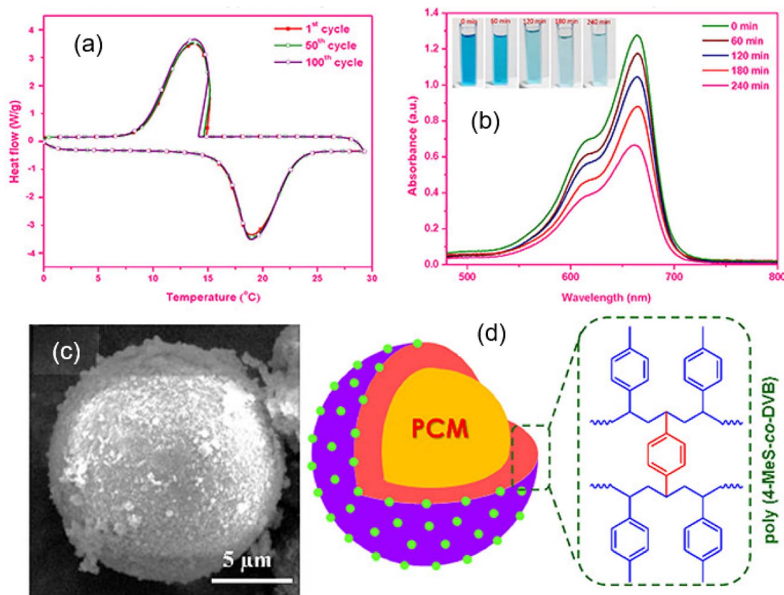
Fig. 8 (a) DSC thermograms of the MPCM [with a TiO 2 decorated poly(4-methylstyrene- co -divinylbenzene) shell and hexadecane PCM] showing thermal cycling capability with 2.6 wt% TiO 2 . (b) UV-visible absorbance spectra of the MPCM sample containing 2.6 wt% TiO 2 . (c) SEM image of the MEPCM, and (d) schematic illustration of the chemical structure of the polymer employed to prepare the MPCM with the decoration of TiO 2 into the shell. Reproduced with permission from ref. 47 Copyright 2021 ACS.
