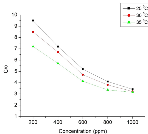
Fig. 10 Langmuir adsorption isotherm ( C/\theta ) versus concentration of \text{Co}_3\text{O}_4 @PPy NCs at 25, 30, and 35 °C.
