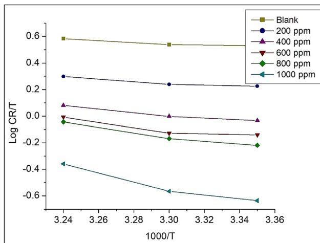
Fig. 9 Plot of log CR/T versus 1000/T for \text{Co}_3\text{O}_4 @PPy NCs.
