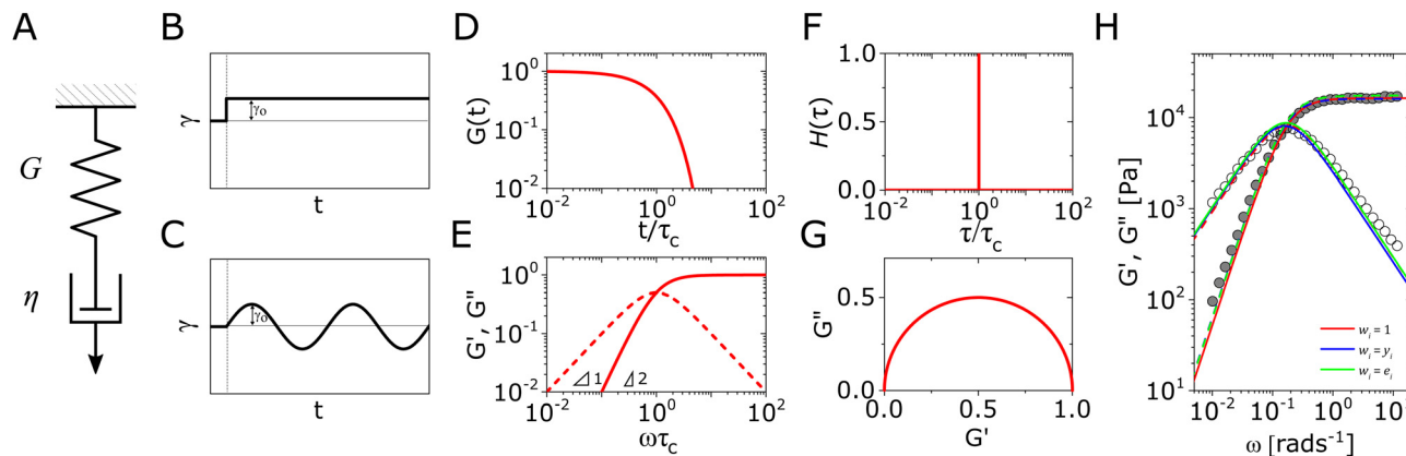
Fig. 1 The Maxwell model of linear viscoelasticity. (A) The Maxwell model consists of a spring with an elasticity of G , and a dashpot with viscosity of \eta , arranged in series. (B) and (C) Illustration of the step strain and oscillatory strain input for studying viscoelastic properties of soft matter, and (D) and (E) corresponding linear viscoelastic responses of the Maxwell model under step strain and oscillatory strain ( G_0 = 1 ). (F) The relaxation spectrum of H(\tau) for the Maxwell model, represented by a delta function centered around \tau = \tau_c . (G) A Cole–Cole plot of the loss modulus G''(\omega) as a function of the storage modulus G'(\omega) . (H) Transient polymer networks as an example of soft materials exhibiting near-Maxwellian viscoelasticity. This particular example shows the viscoelastic response of a metal-coordinating transient polymer network consisting of histidine-functionalized poly(ethylene glycol) with \text{Ni}^{2+} ions. 13 Here we also demonstrate this fitting process using three different weights in the residual function – see eqn (26) in Section VI and discussion thereof – which leads to a statistical difference in the values of the final fitting parameters.
