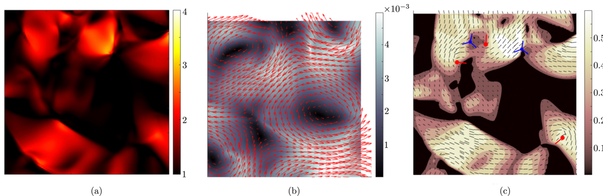
Fig. 4 Fully developed active turbulence with deformable particles. (a) Aspect ratio, \omega of particles. (b) Velocity field, u . Colour scale indicates the magnitude of the velocity. (c) Nematic director field \mathbf{n} and scalar order parameter S . Colour scale indicates the magnitude of S . Red/blue symbols correspond to the core of \pm 1/2 defects respectively. +1/2 defects are oriented such that the tail is along the line shown.
