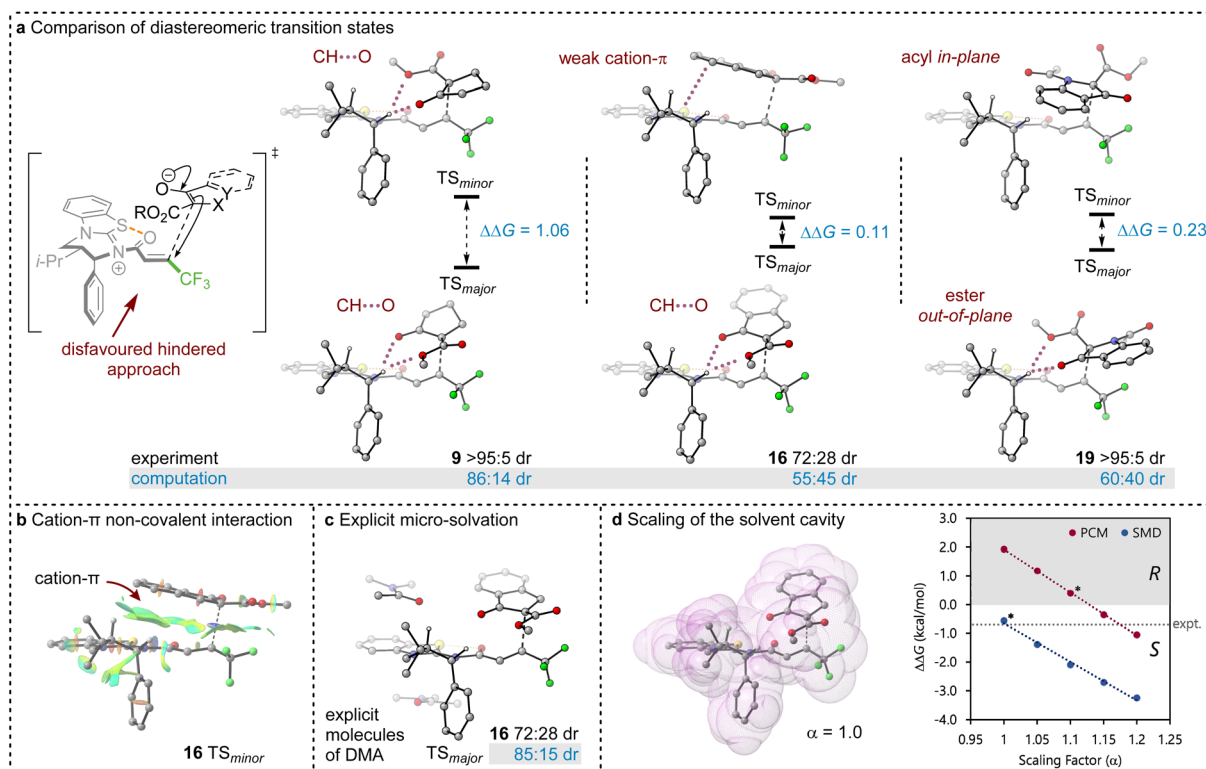
Fig. 1 (a) DFT analysis of the most stable major and minor diastereomeric transition states. Important interactions are highlighted, with dual CH...O interactions present in all major TS. M06-2X SMD /def2-TZVP//M06-2X SMD /def2-SVP free energies ( \Delta G_{298} ) are shown in kcal mol -1 and selected hydrogen atoms have been removed for clarity. (b) Non-covalent interaction of key cation- \pi stabilisation of minor diastereomeric TS of 16 . (c) Explicit micro-solvation with \pi -type interaction with conjugated DMA solvent (with PCM solvation model). (d) Solvent cavity as a sum of van der Waals radii and graph of the selectivity ( \Delta\Delta G_{298} ) as a function of the scaling parameter. Asterisks indicate the default value of \alpha for each solvent model.
