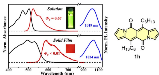
Fig. 14 Normalized absorption (black) and fluorescence (red) spectra of DPND in \text{CH}_2\text{Cl}_2 solution ( 10^{-5} M) and solid thin film (100 nm), as well as sensitized phosphorescence spectra (blue) of 1h in polystyrene (PS) matrix (DPND : PtTPBP : PS = 1 : 5 : 94) and doped thin film (DPND : PtTPBP = 95 : 5). Inset: sample photographs of solution and thin film under 365 nm UV light. Adapted with permission from ref. 8d. Copyright 2020 American Chemical Society.
