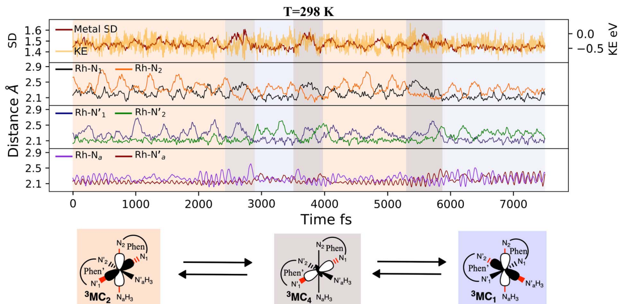
Fig. 3 ^3\text{MC} AIMD trajectories for 7500 fs at 298 K. (top panel) metal spin density (SD) in red and kinetic energy (KE in eV) fluctuations in yellow. (middle panels) metal–ligand bond distances (in Å) for phen (black and yellow), phen' (blue and green), and the two amine groups (purple and red).
