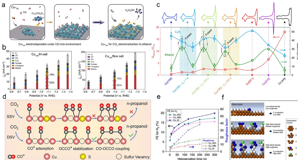
Fig. 9 (a) Schematic illustration of the synthesis of a Cu DS catalyst under a CO-rich environment, which favours high coverage of the *CO intermediate and promotes alcohol production, and the subsequent CO 2 RR process. (b) The product distribution of the Cu DS catalyst in an H-type cell and flow cell, respectively. Reproduced from ref. 177. Copyright 2021 Elsevier. (c) Q_{\text{defects}}/Q_{100} and product selectivity as a function of pulsed versus potentiostatic conditions on a Cu(100) electrode; copper stepped surfaces were used for comparison. Voltammetric properties of the copper surfaces recorded in 0.1 M NaOH ( 50 \text{ mV s}^{-1} ) are shown in the top row. Unless otherwise stated, measurements were performed at a constant potential of -1.0 \text{ V} , and the pulse conditions are labelled as: E_a = 0.6 \text{ V} , E_c = -1.0 \text{ V} , t_a = 1 \text{ s} , t_c as indicated, 1 h reaction. Measurements performed under pulsed conditions and continuous constant potential are indicated by shaded areas. Reproduced from ref. 178. Copyright 2020 Nature. (d) Schematic illustration of the formation mechanism of n -propanol on the adjacent Cu x -DSV, showing the dimerization of CO-CO and coupling of CO-OCCO. Reproduced from ref. 98. Copyright 2021 Nature. (e) Diagram of catalyst roughness and FE of H 2 as a function of halogenation time. (f) Schematic diagram of low coordination copper atoms and surface roughness with the corresponding ECR results. The coordination number for face-centred cubic copper is 12. Reproduced from ref. 180. Copyright 2020 Nature.
