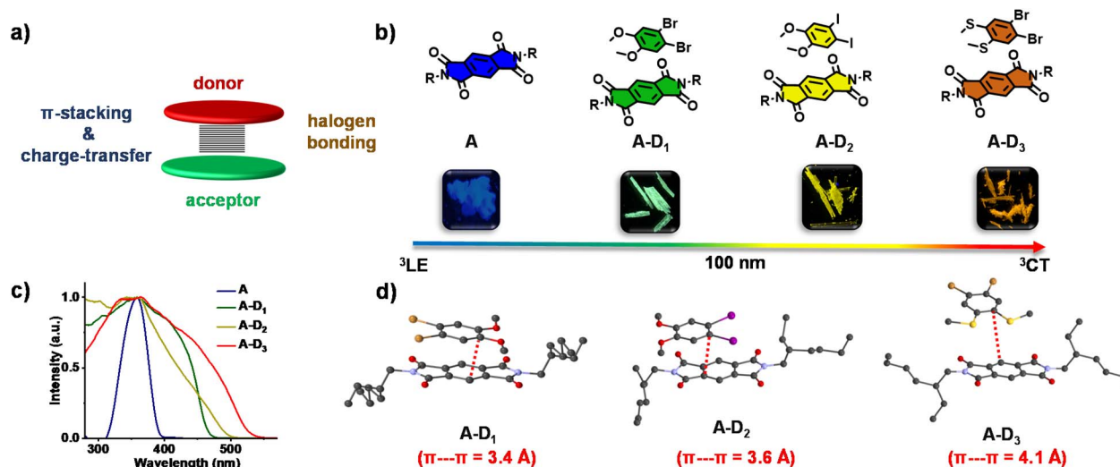
Fig. 1 (a) Schematic illustrating the design of non-covalent donor-acceptor cocrystals. (b) Molecular structures of pyromellitic diimide ( A ) and corresponding donor-acceptor cocrystals ( A - D 1 , A - D 2 and A - D 3 ) with the photographs of their cocrystals (under a 365 nm UV lamp) and emission of A and the corresponding cocrystals ( A - D 1 , A - D 2 and A - D 3 ) showed a clear red-shift of 100 nm from cyan to green to yellow to reddish orange. (c) Excitation spectra of A ( \lambda_{\text{monitored}} = 500 nm) and corresponding cocrystals ( A - D 1 , A - D 2 and A - D 3 ; \lambda_{\text{monitored}} = 515 nm, 555 nm and 595 nm, respectively), which showed a red-shifted band compared to A , signifying the CT interaction. (d) Single-crystal X-ray diffraction data showing the \pi - \pi interactions and corresponding distances (shown in red dashed lines) in cocrystals.
