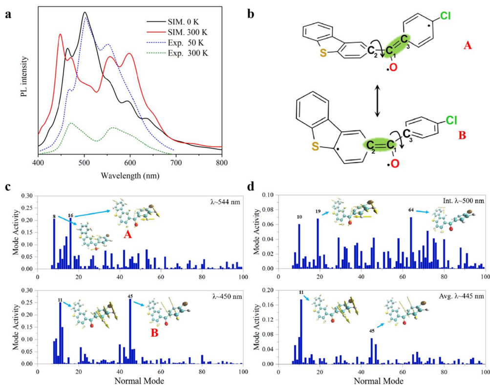
Fig. 4 Simulated spectra and vibration analysis, (a) the simulated phosphorescence spectra of 3_{\text{CIBDBT}} with the temperature of 0 K (solid black line) and 300 K (solid red line) in comparison with experimental spectra of 50 K (dot blue line) and 300 K (dot green line); (b) two mesomerism structures of A and B; coherent activity of the vibrational normal modes for (c) structures with PL bands ( \lambda ) at ca. 544 and 450 nm, respectively, from Wigner sampling at 300 K, and (d) structures from QM/MM MD simulations at 300 K of initial structure ( \lambda = 500 nm) and the averaged structure ( \lambda = 445 nm). The most active modes are represented as an inset. The simulated spectra are shifted by -0.14 eV in order to be consistent with experimental observations.
