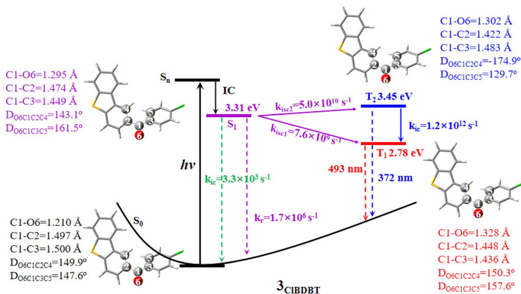
Fig. 3 The adiabatic energy levels, radiative ( k_{\text{r}} ) and nonradiative ( k_{\text{ic}} and k_{\text{isc}} ) rates, as well as T 1 and T 2 emission wavelengths for 3_{\text{CIBDBT}} . The ground state energy (-1660.75414666 a.u.) of 3_{\text{CIBDBT}} is set as the reference at the CC2/cc-pVDZ level. The geometrical parameters for some important bonds and dihedral angles are also shown.
