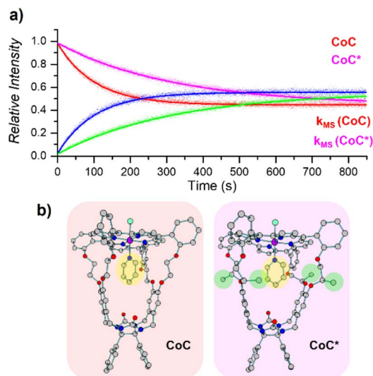
Fig. 6 (a) Relative time evolution of [\text{CoC}(\text{Py})]^+ (red), [\text{CoC}(\text{Py})_{\text{OUT}}]^+ (blue), [\text{CoC}^*(\text{Py})_{\text{OUT}}]^+ (magenta), and [\text{CoC}^*(\text{Py})_{\text{IN}}]^+ (green) in a single DRL experiment carried out at 40 °C in \text{CHCl}_3 with 200 equiv. pyridine and 200 equiv. pyridine-D5. Dots are experimental data points, and lines correspond to fittings of experimental data by eqn (S1) and (S2). † (b) DFT-calculated structures of ^1[\text{CoC}(\text{Cl}_{\text{OUT}})(\text{Py}_{\text{IN}})] and ^1[\text{CoC}^*(\text{Cl}_{\text{OUT}})(\text{Py}_{\text{IN}})] optimized with B3LYP-D3/def2svp.
