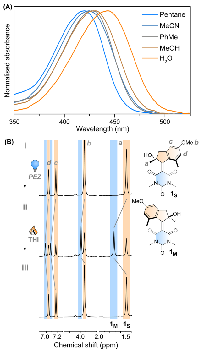
Fig. 2 (A) Normalised UV-vis absorption spectra of 1_s in different solvents. (B) ^1\text{H} NMR irradiation studies of 1_s in \text{CD}_3\text{OD} ( c = 1 \times 10^{-3} \text{ M} ) at -90^\circ\text{C} . (i) 1_s before irradiation; (ii) \text{PSS}_{420} , 63 : 37 ( 1_M : 1_S ); (iii) \text{TH1} , -45^\circ\text{C} , 15 min.
