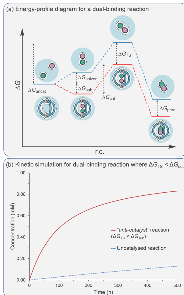
Fig. 8 (a) Energy profile diagram for a cage-mediated dual-binding reaction. (b) Kinetic simulation of a dual binding reaction where stabilisation of the substrates, \Delta G_{\text{sub}} , is greater than stabilisation of the TS, \Delta G_{\text{TS}} . Simulation conditions: [\text{subA}]_0 = [\text{subB}]_0 = [\text{cage}]_0 = 1 \text{ mM} ; k_{\text{subA-on}} = k_{\text{subB-on}} = 1.0 \times 10^{11} \text{ M}^{-1} \text{ s}^{-1} ; k_{\text{subA-off}} = k_{\text{subB-off}} = 1.0 \times 10^6 \text{ s}^{-1} ; K_{\text{TS}} = 3.3 \times 10^8 \text{ M}^{-1} ; K_{\text{prod}} = 0 \text{ M}^{-1} ; k_{\text{uncat}} = 0.30 \text{ M}^{-1} \text{ s}^{-1} ( \Delta G_{\text{uncat}} = 23 \text{ kcal mol}^{-1} ); k_{\text{cat}} = 0.01 \text{ s}^{-1} ( \Delta G_{\text{uncat}} = 25 \text{ kcal mol}^{-1} ).
