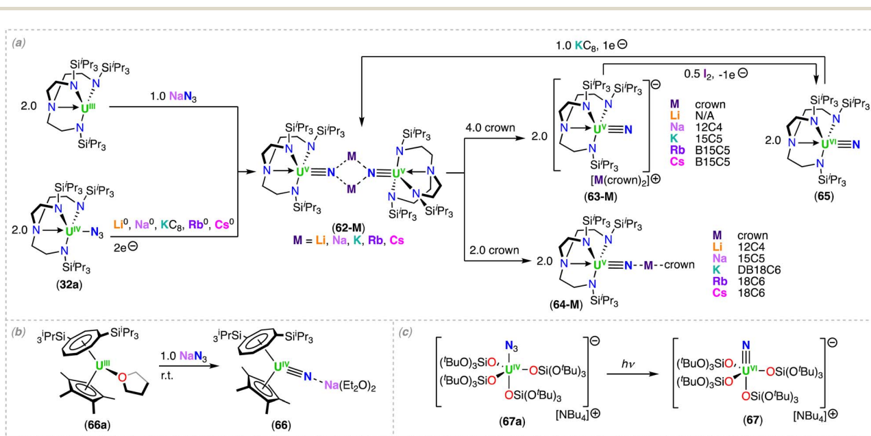
Scheme 13 Synthesis of (a) alkali-capped and terminal uranium-nitrides supported by the triamidoamine ( \text{Tren}^{\text{TIPS}} ) ligands; (b) organometallic alkali-capped uranium(V)-nitride; (c) terminal uranium(VI)-nitride supported by siloxide ( -\text{OSi}(\text{O}^t\text{Bu})_3 ) ligands.
