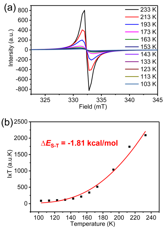
Fig. 6 (a) VT ESR spectra and (b) fitted \ln T vs T curves by using the Bleaney–Bowers equation of carbonylated cycloarene diradical K3-R in a solid.
