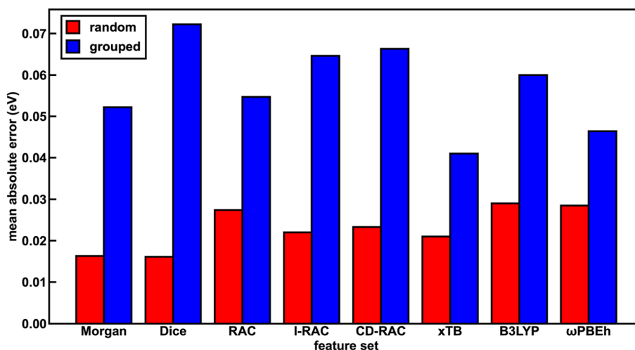
Fig. 2 The test set performance of ANNs trained on different feature sets in predicting Em_{50/50} (MAE, in units of eV) for both random (red bars) and grouped splits (blue bars). Here, I-RAC refers to ligand-only RACs.
